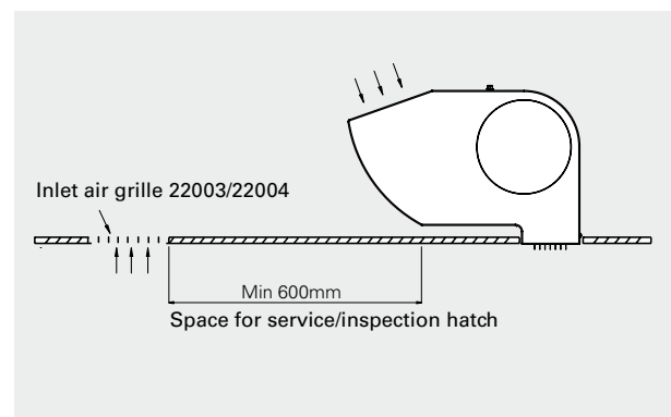
Fig. 2: False ceiling mounting
